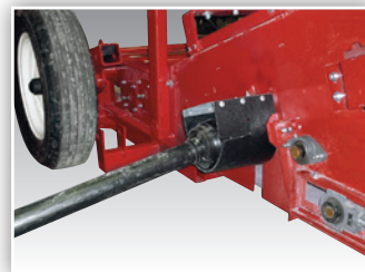
PTO Drive
