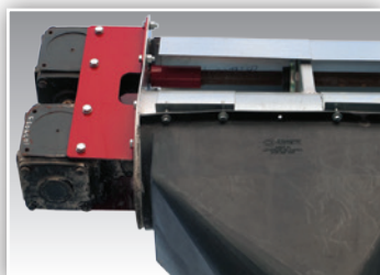
DOUBLE OIL BATH GEARBOX HEAD DRIVE
